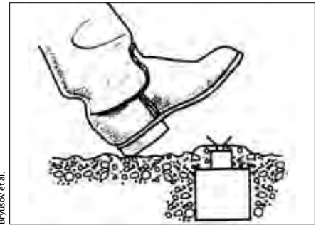
Figure 21.2.2 Mechanism of detonation of a blast mine.
